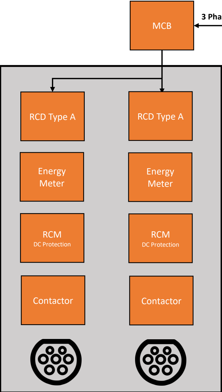
Dual-Port Wallbox - Option 1 (22KW Shared Supply, 2.5 to 4mm core cable inside)
